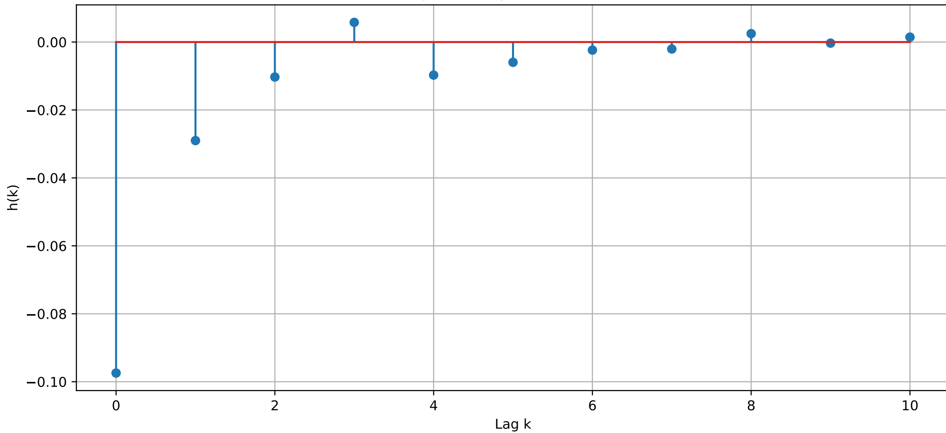
Impulse Response: Gv \rightarrow Ph
