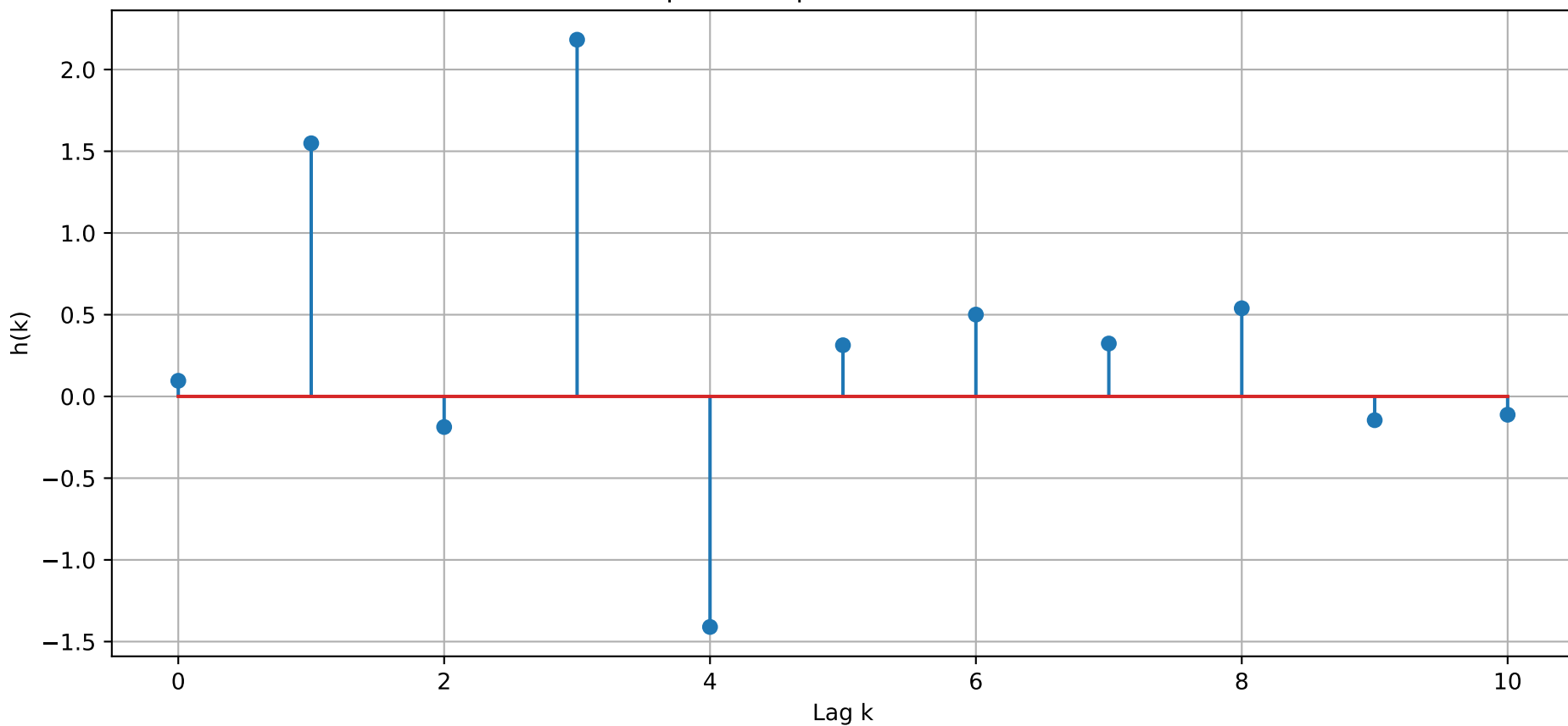
Impulse Response: Gv \rightarrow Ph
